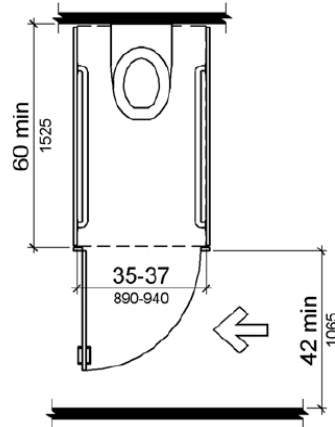
Figure 604.8.2 Ambulatory Accessible Toilet Compartment
